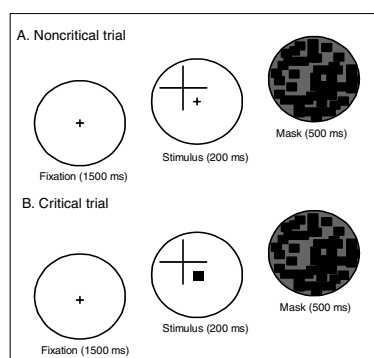
Fig. 1. The experimental protocol related to the discovery by Mack and Rock of inattention blindness
